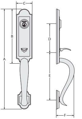
HANDLESET - 3/4 & FULL DIMENSIONS
